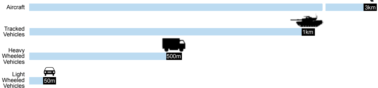
Acoustic detection and tracking ranges
